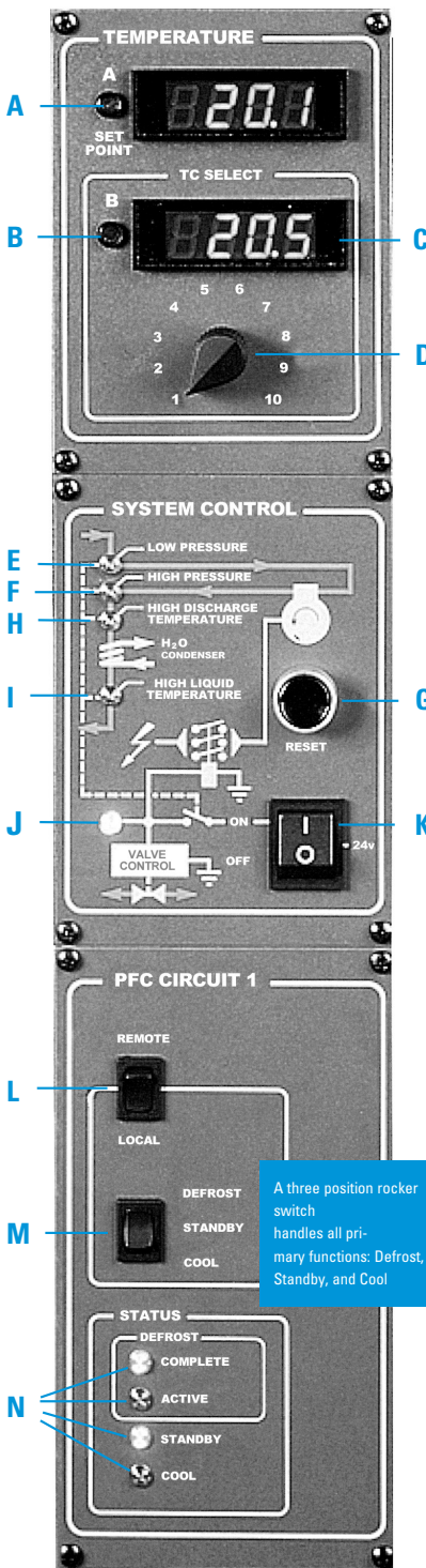
Model PFC Control Panel
