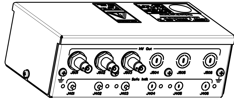
410012-3 3 WAY SPLITTER
